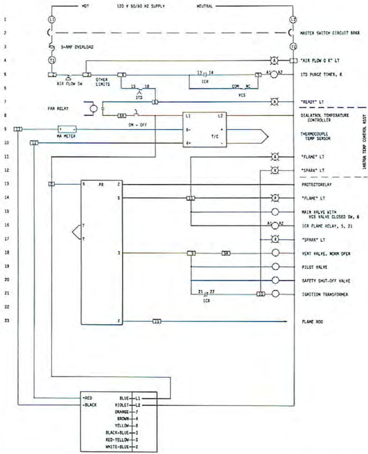
BARBER-COLMAN MODULATING MOTOR
